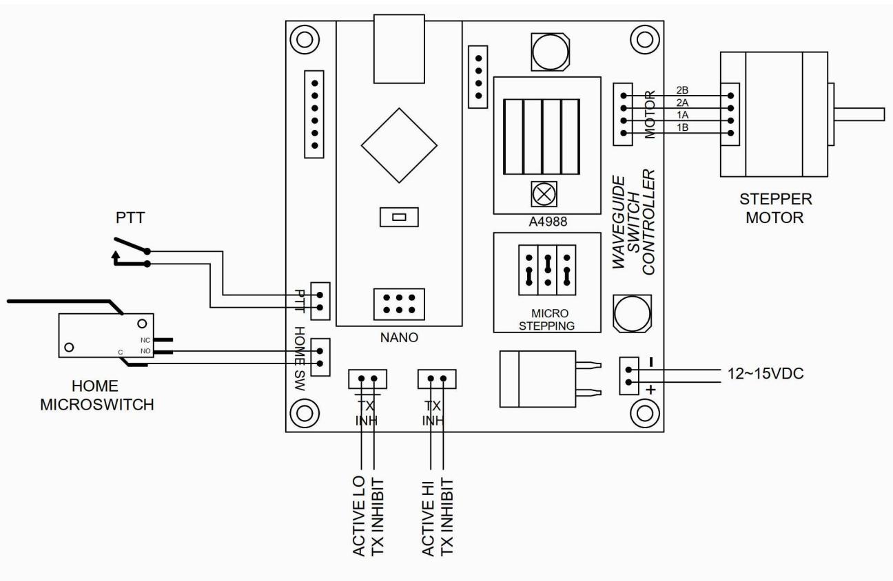
CONNECTION DIAGRAM
